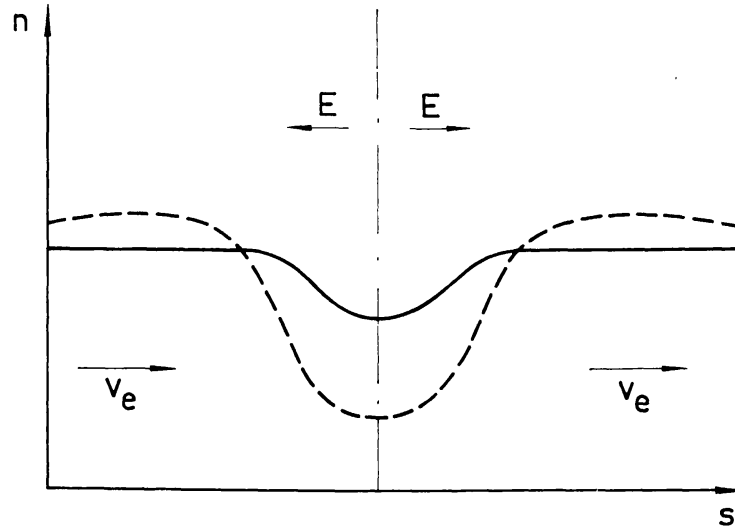
Fig. 3. Particle density n=n_e=n_i given as a function of the distance s . The solid line shows the initial state indicating a small density dip, and the dashed curve shows the configuration at a later time. The electrons move to the right with the velocity v_e . Acceleration and retardation of the electrons are produced by an electric field E .
